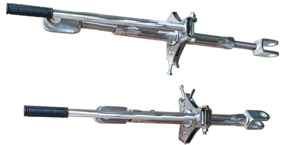
Derrick Angle Adjustment Assembly
